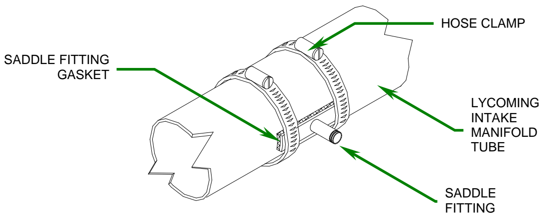
FIGURE 2-3 - SADDLE FITTING INSTALLATION (LYCOMING W/O CUFF)
