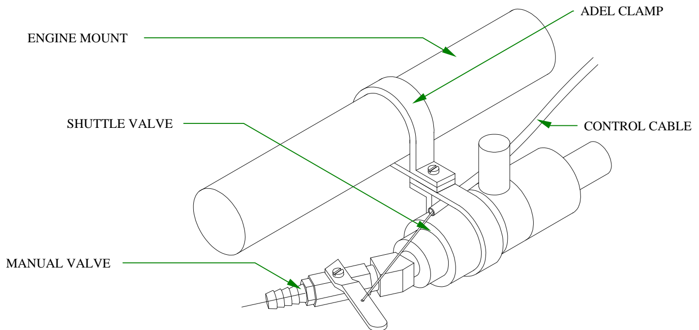
FIGURE 2-1 - SHUTTLE VALVE INSTALLATION
