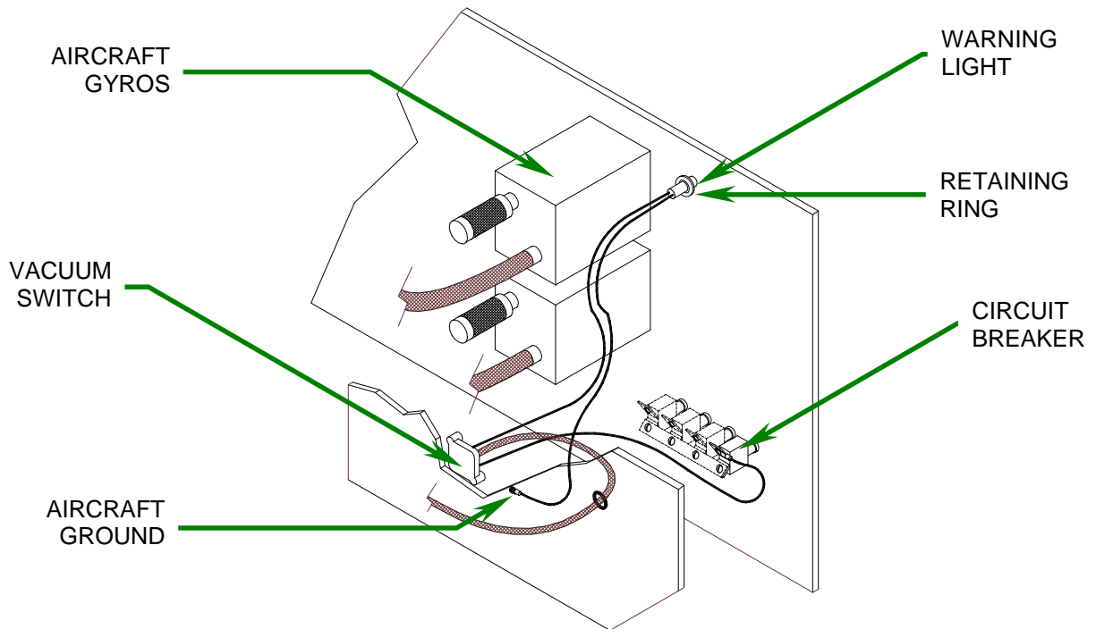
FIGURE 2-7 - WARNING LIGHT INSTALLATION
