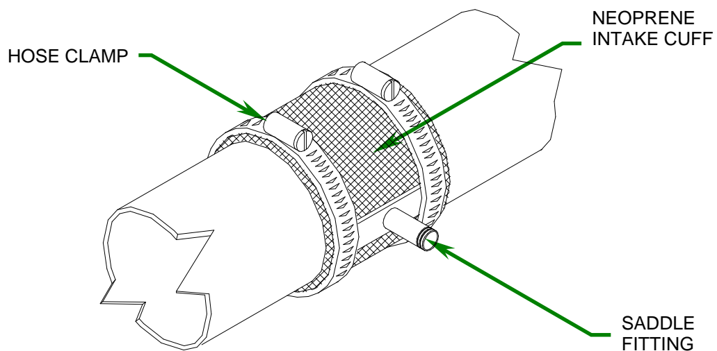
FIGURE 2-2 - SADDLE FITTING INSTALLATION
