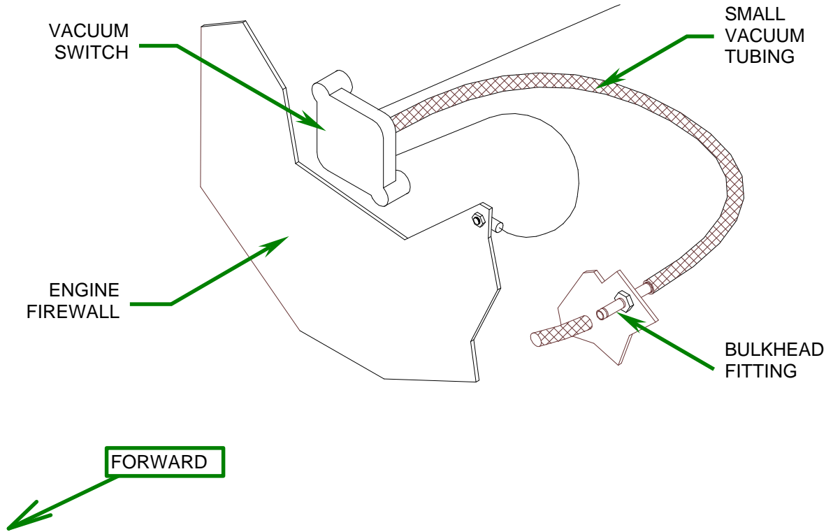
FIGURE 2-4 - VACUUM SWITCH INSTALLATION
